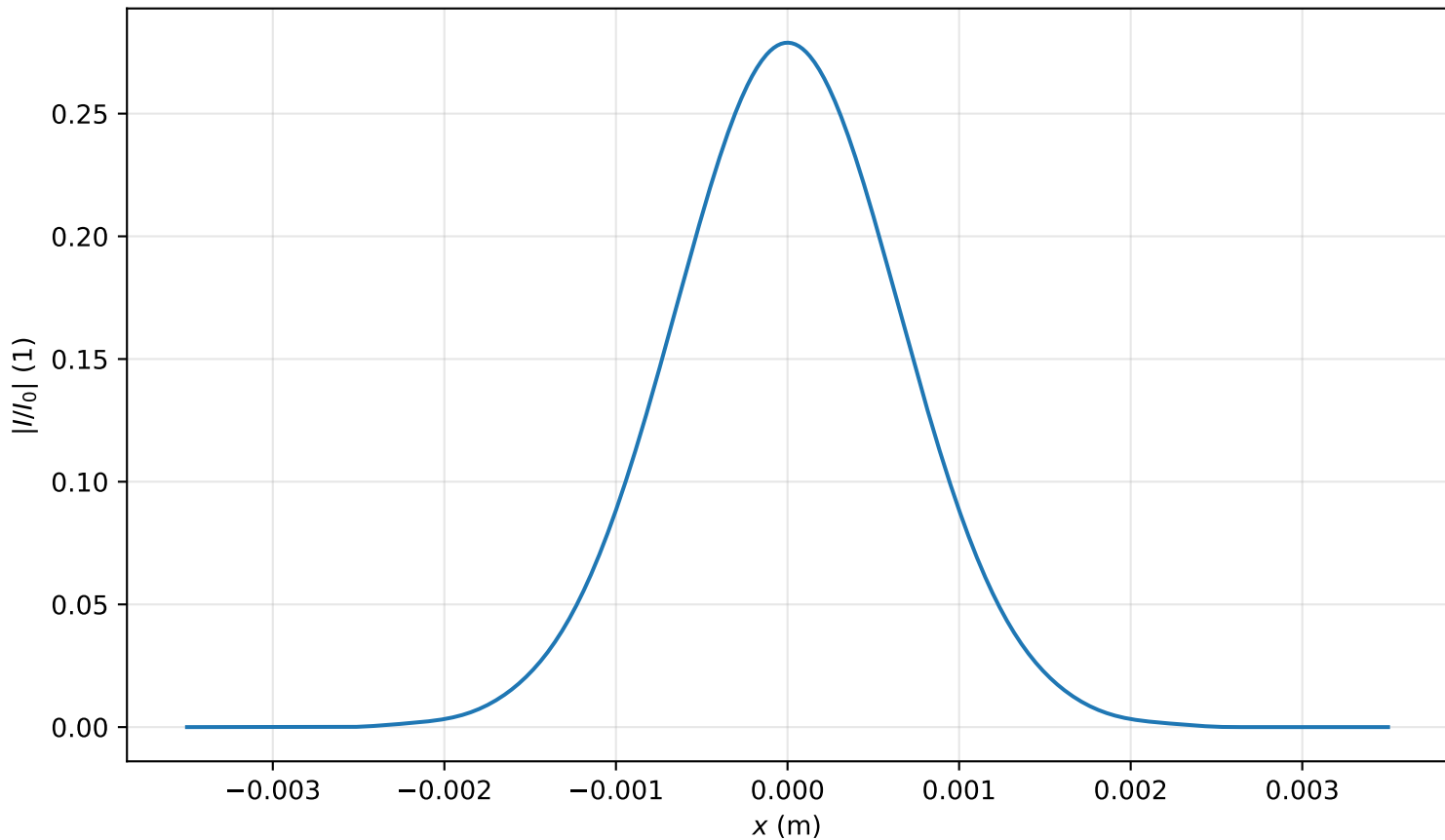
Intensity profile I(x, y = 0, z = 3.423m)/I_0 , P_{in}=0.1P_{cr} , artificial time
